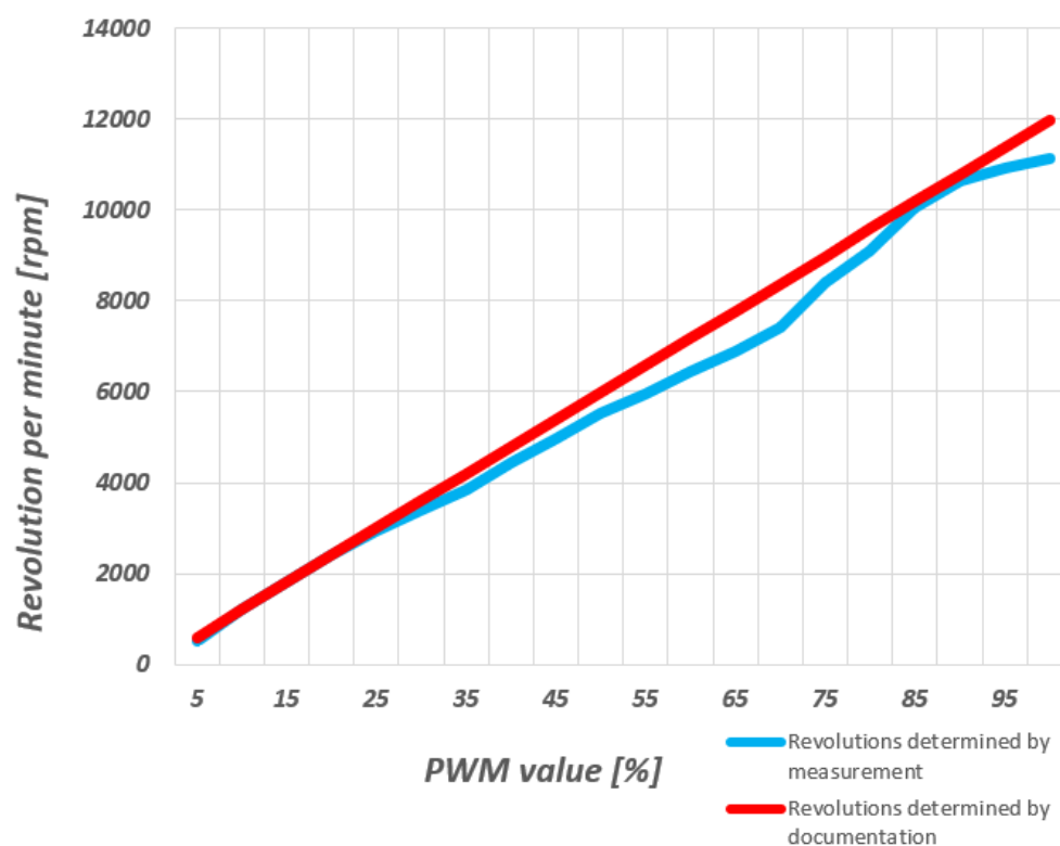
Figure 4. Ideal and calculated motor speed characteristics for PWM values, measurements carried out at 12.60V
