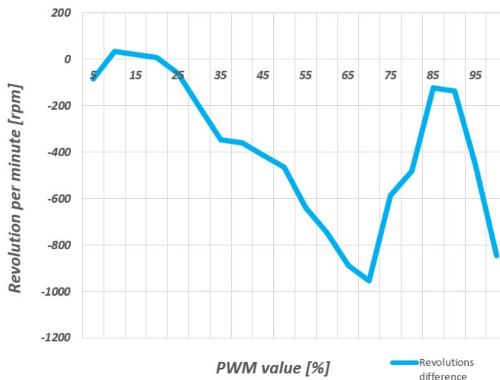
Figure 5. Presentation of difference values between revolutions determined by documentation and revolutions determined by measurements
