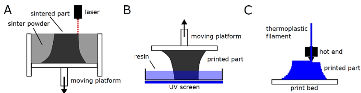
Figure1. 3D printing methods: A – Selective Laser Sintering, B – Digital Light Processing, C – Focused Deposition Modeling [5]
