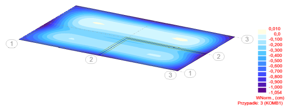
Figure 6. Map of the deflection of the foundation slab in the Z direction [13]
