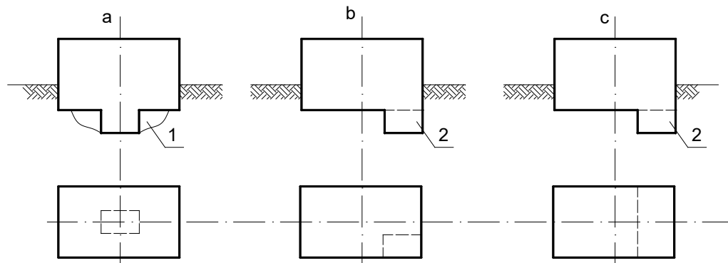
Figure 1. Examples of variants for shaping the foundations of buildings at different depth levels: a – central recess, b and c – asymmetrical recess of the building section; 1 – compacted sand or lean concrete, 2 – horizontal expansion joint with slip layer [11], [12]
