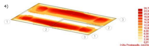
Figure 8. Reinforcement compaction maps: 1) bottom in direction X, 2) 1) bottom in direction Y, 3) top in direction X, 4) top in direction Y, (ROBOT program option - theoretical selection of reinforcement) [13]
