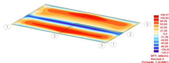
Figure 5. Map of bending moments in the YY direction [13]
