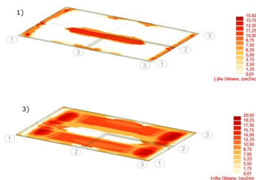
Figure 8. Reinforcement compaction maps: 1) bottom in direction X, 2) 1) bottom in direction Y, 3) top in direction X, 4) top in direction Y, (ROBOT program option - theoretical selection of reinforcement) [13]
