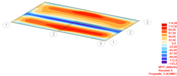
Figure 10. Map of bending moments in the YY direction – variant II [13]
