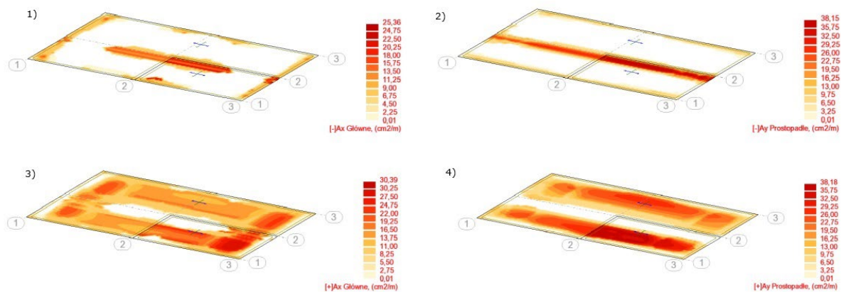
Figure 13. Reinforcement compaction maps: 1) bottom in direction X, 2) 1) bottom in direction Y, 3) top in direction X, 4) top in direction Y, (ROBOT program option – theoretical selection of reinforcement) [13]
