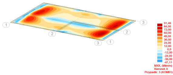
Figure 9. Map of bending moments in the XX direction variant II [13]
