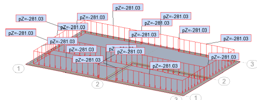
Figure 3. Load combination taking into account slab weight and load from bearing walls [13]
