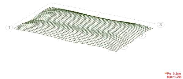
Figure 12. Deformation of a slab working on elastic substrate with simulated collapse under part of the object – variant II [13]
