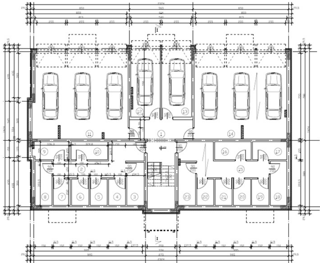
Figure 2. Basement drawing of the designed building [13]
