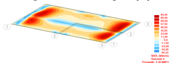
Figure 4. Map of bending moments in the XX direction [13]
