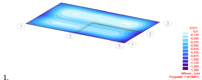
Figure 11. Map of the deflection of the foundation slab in the Z direction – variant II [13]
