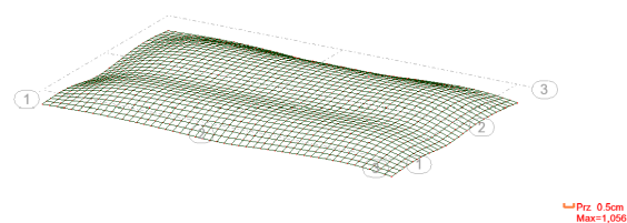
Figure 7. Deformation of the foundation slab working on elastic ground [13]
