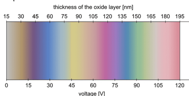
Figure 5. Graph showing the colors obtained depending on the voltage used and the thickness of the oxide layer [8]
