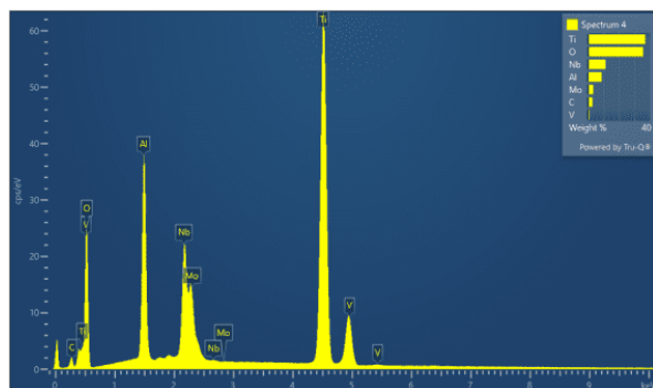
Figure 14. EDS analysis for the sample oxidized during 300h
