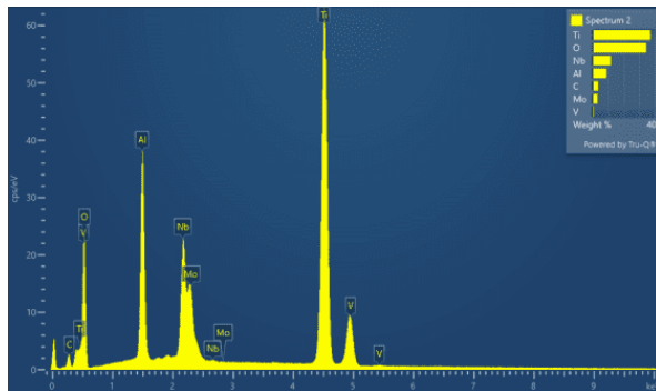
Figure 13. EDS analysis for the sample oxidized during 100h
