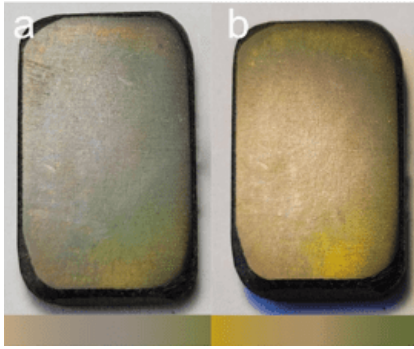
Figure 9. Surface of the oxidized sample during 300 h; a) in cold light, b) in warm light
