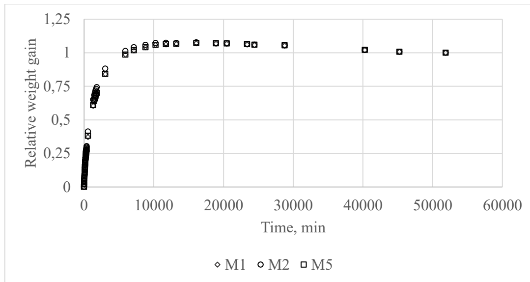
Figure 6. Relative weight gain over time – soft wool, RH range 45 to 90%
