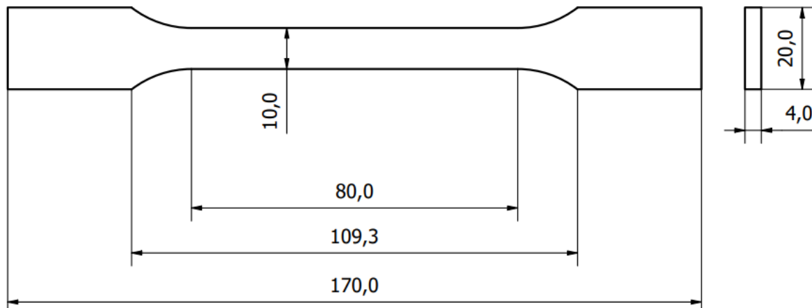
Figure 1. Dimensions of a test sample in compliance with the PN-EN ISO 527-1:2012 standard jaws
